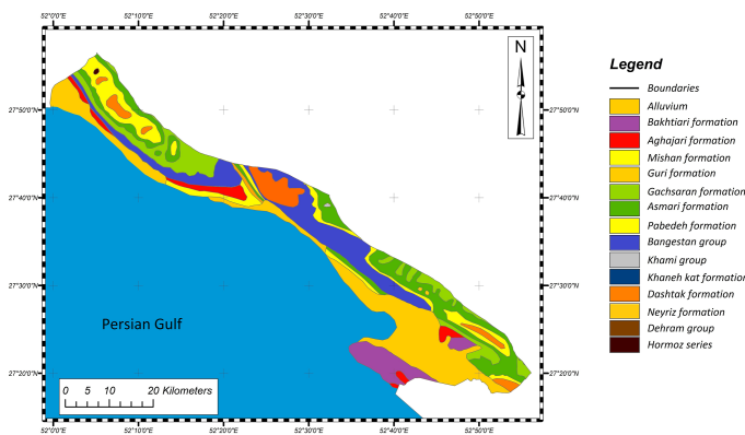
Fig. 6 Geology map of studied location (Azarafza et al., 2018b)
